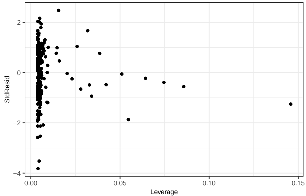
Ca WLS_weighted - Leverage Plot
